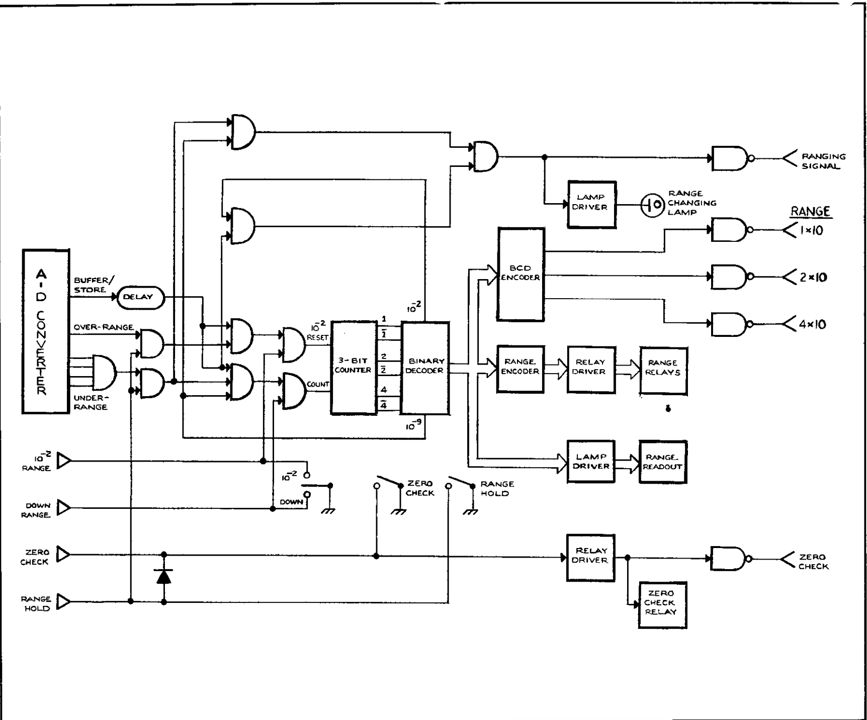
FIGURE 12. Autorangeing Block Diagram.
