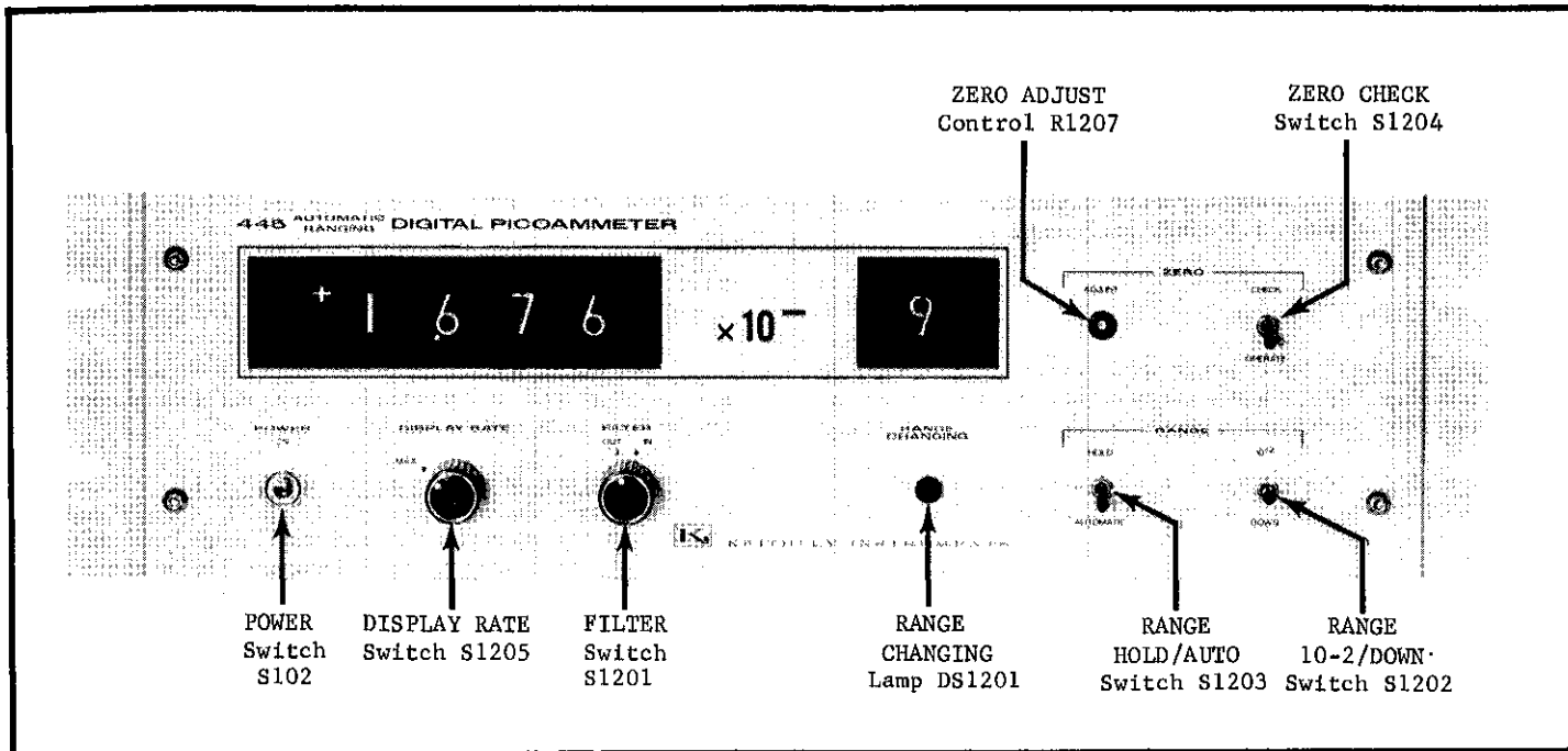
FIGURE 2. Front Panel Controls.
