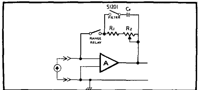
FIGURE 10. Range Calibration.
