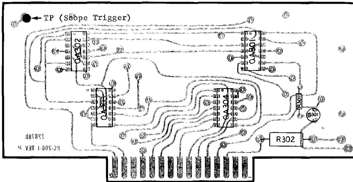
FIGURE 21. Component Layout, PC-208.
