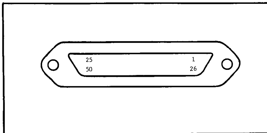
FIGURE 7. Printer/Control Connector.
