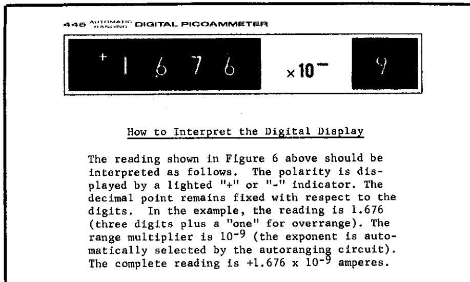
FIGURE 6. Digital Display.
